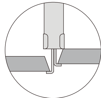
internal misalignment
