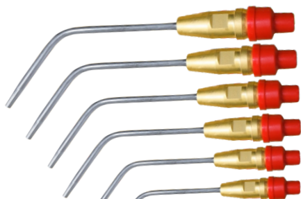
Welding nozzle X21-W (1,2,3,4,5,6)
